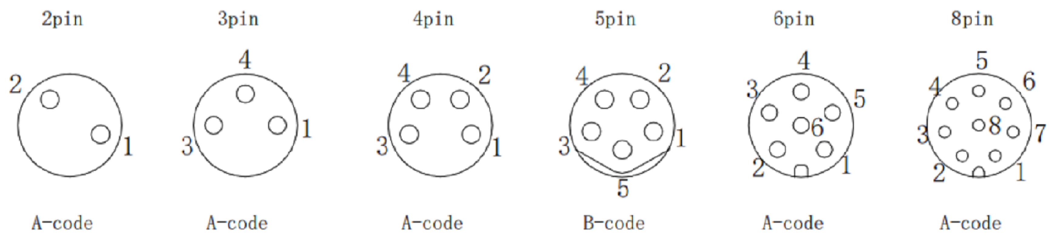
Pin assignment front view/针位分布前视图
